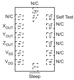
Figure 4. Pinout Description
