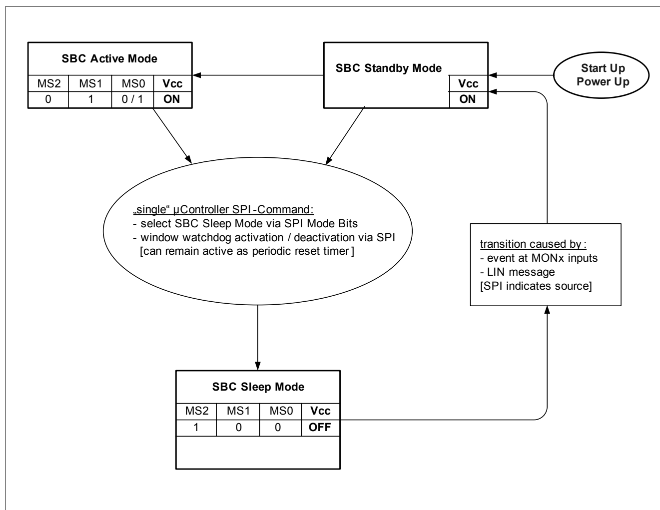
Figure 6 State Diagram "SBC Sleep Mode"
