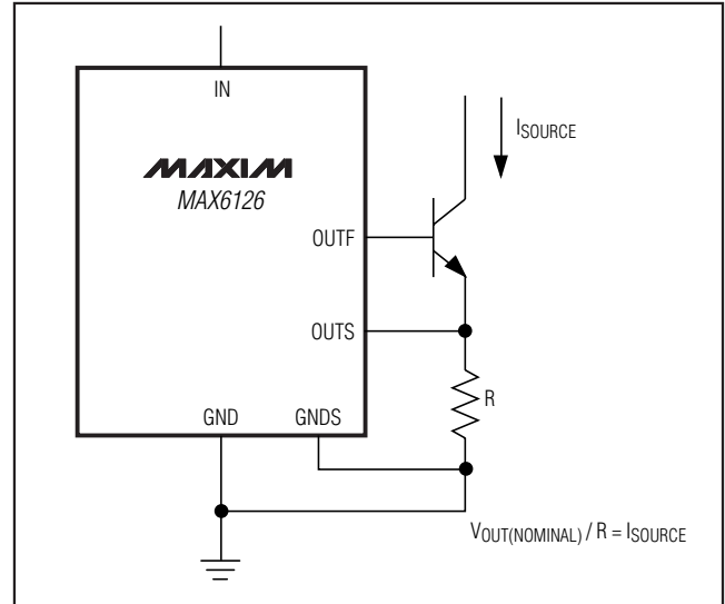
Figure 2. Precision Current Source
