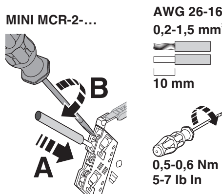
Figure 4 Screw connection
