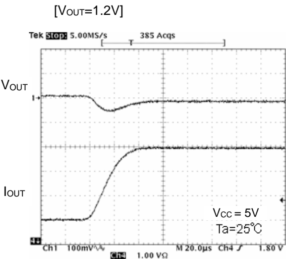
Figure 17. Transient Response (Io=1A to 4A, 20µs)
