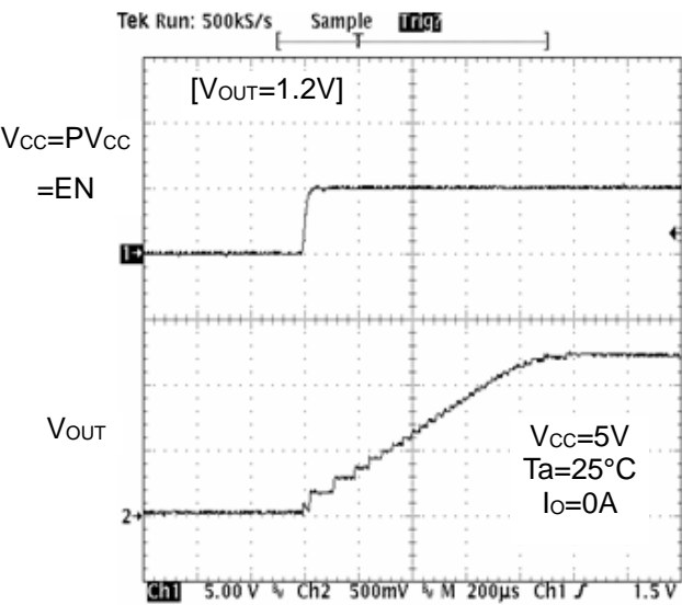
Figure 14. Soft-Start Waveform
