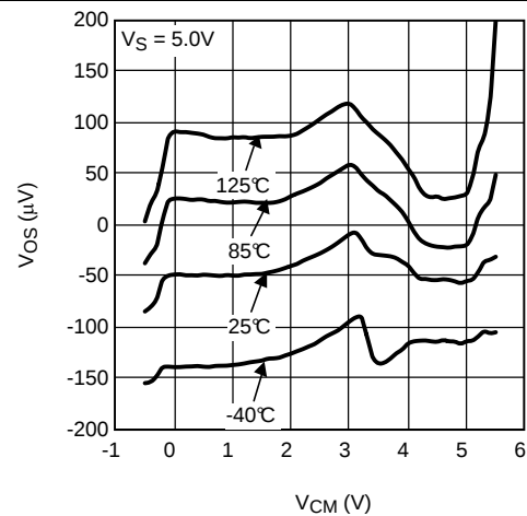
Figure 2. V_{OS} vs V_{CM} Over Temperature at 5 V
