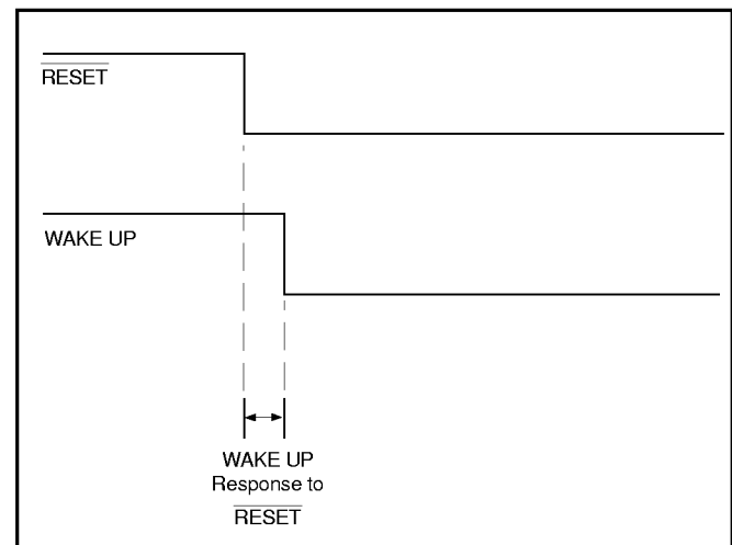
Figure 3. WAKE UP response to RESET (Low Voltage)
