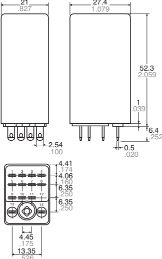
4 Form C External dimensions
