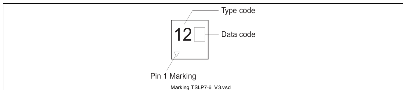
Figure 7 Marking Info
