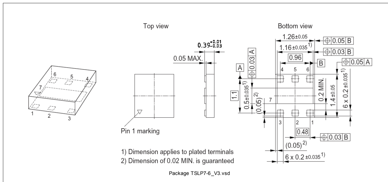
Figure 6 Package TSLP7-6
