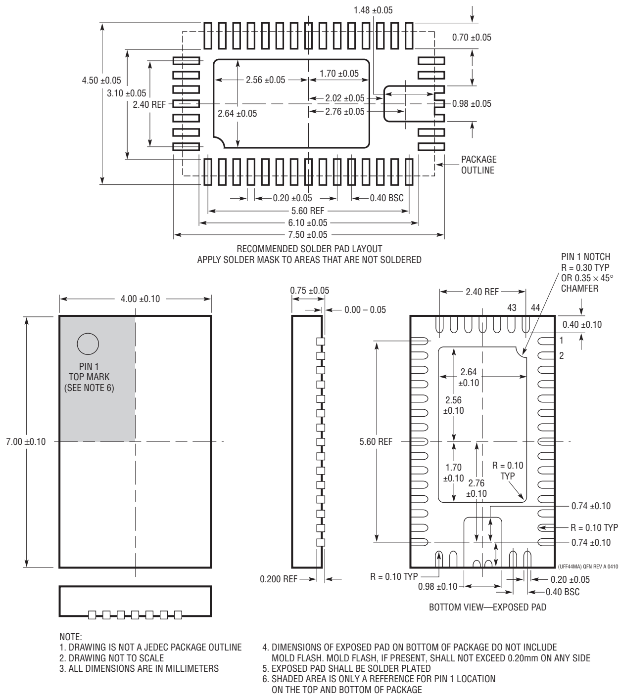
UFF Package Variation: UFF44MA 44-Lead Plastic QFN (4mm × 7mm) (Reference LTC DWG # 05-08-1762 Rev A)
