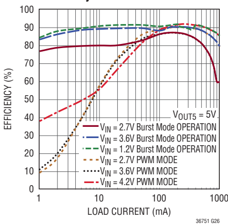
Boost Regulator, Efficiency vs Load
