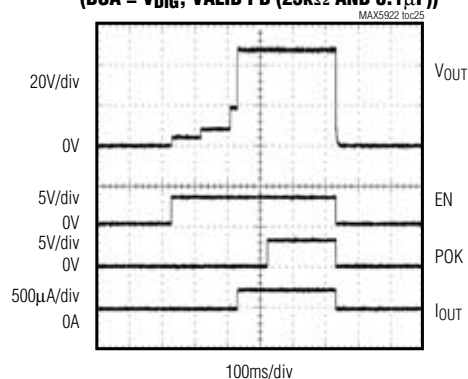
STARTUP WITH MIDSPAN MODE (DCA = V_{DIG} , VALID PD (25k \Omega AND 0.1μF))
