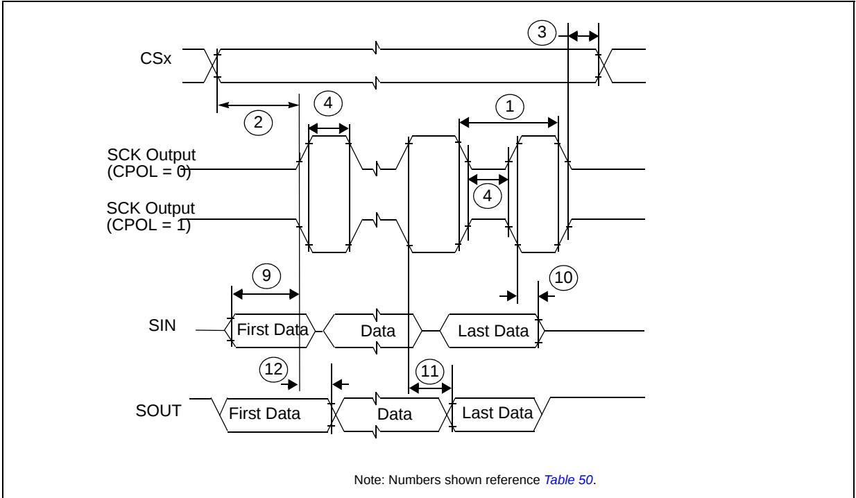
Figure 30. DSPI modified transfer format timing-master, CPHA = 1
