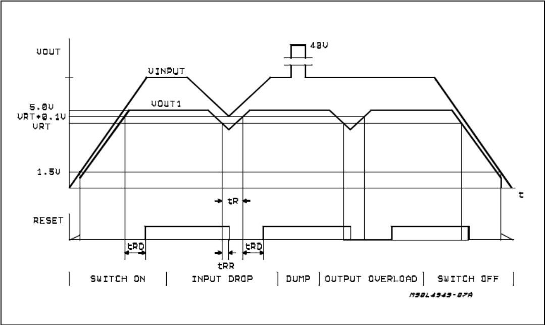
Figure 8. Waveforms
