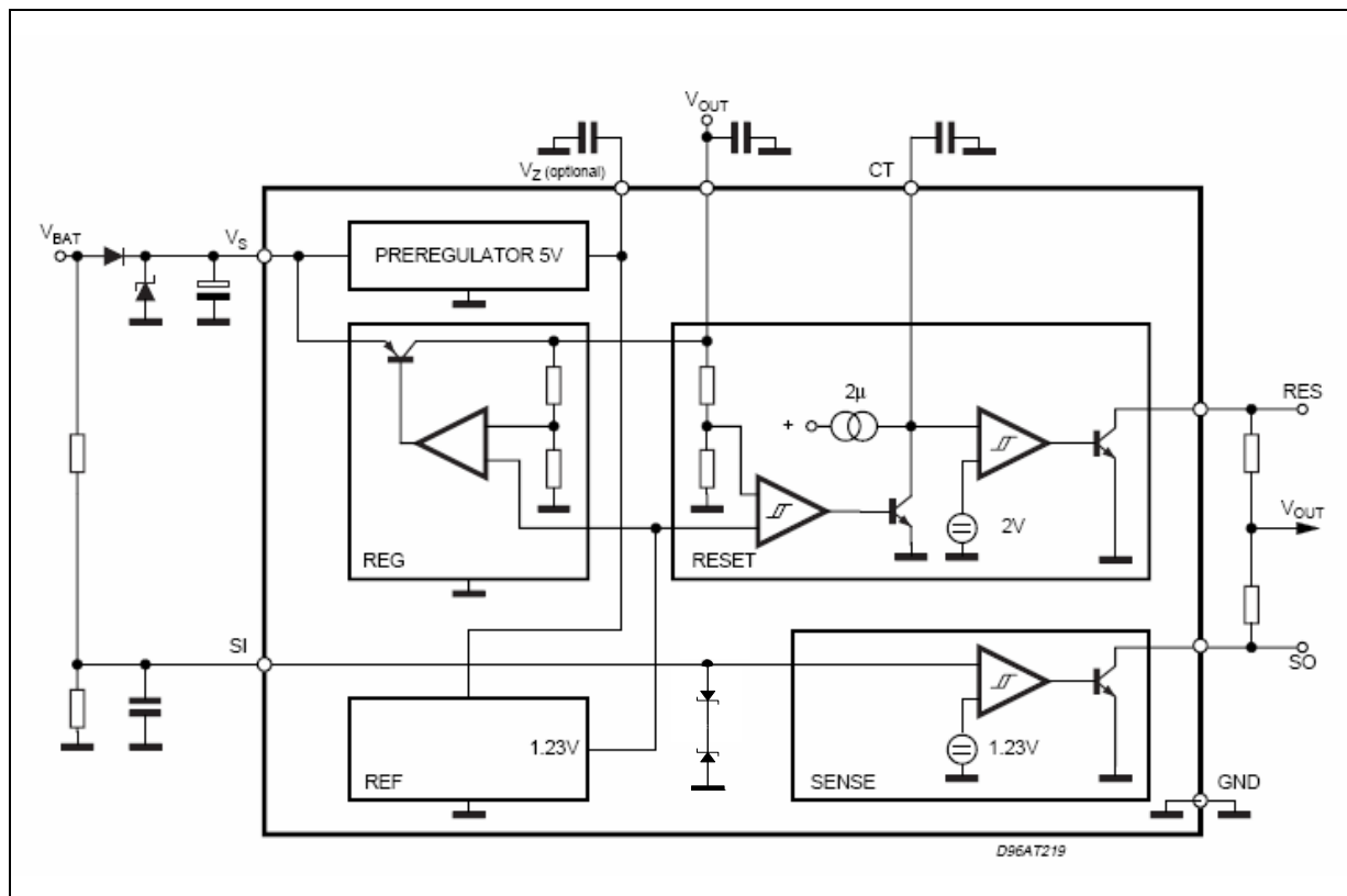
Figure 3. Application circuit
