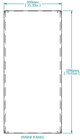
INNER PANEL
