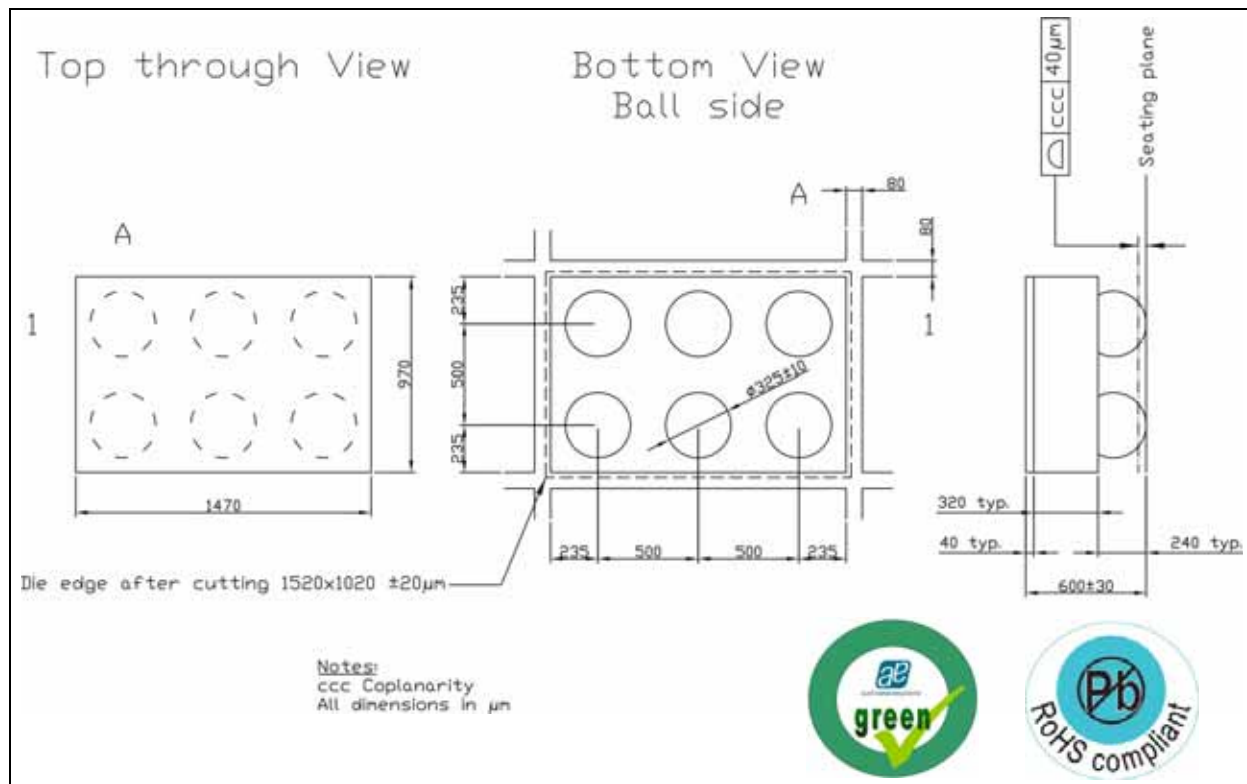
Figure 27. 6-bump WLP Package
