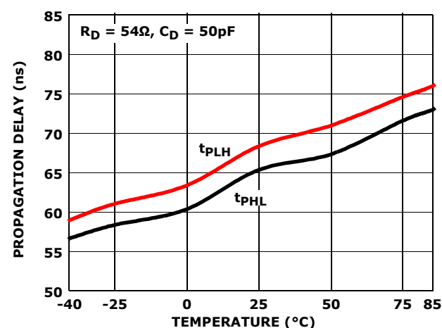
FIGURE 15. DRIVER DIFFERENTIAL PROPAGATION DELAY vs TEMPERATURE (ISL31475E)
