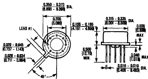
8 Lead TO-99 (TV) \theta_{JA} = 25^{\circ}\text{C/W} \theta_{JC} = 2^{\circ}\text{C/W}
