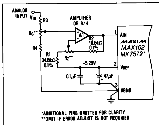
Figure 19. MAX162/MX7572 Non-inverting Bipolar Operation
