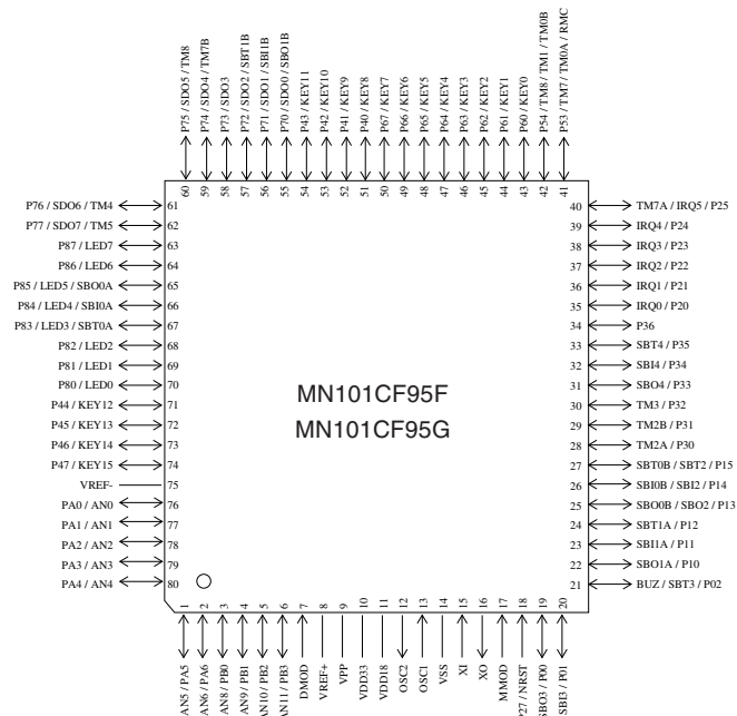
TQFP080-P-1212D *Lead-free
