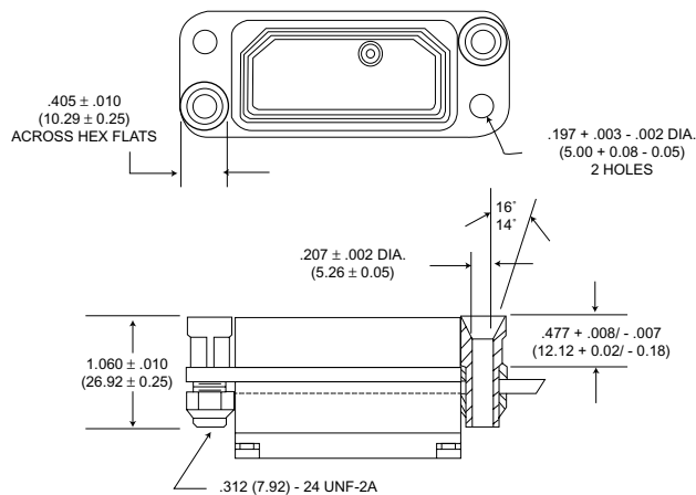
Mounting Style X With Guide Sockets MIL-C-83733/3(USAF)
