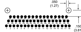
51 Contacts
