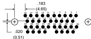
37 Contacts
