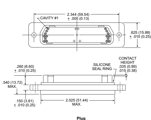
Plug
