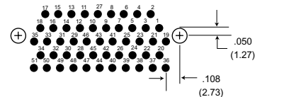
51 Contacts
