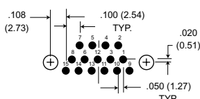
15 Contacts
