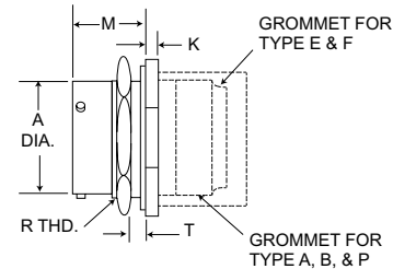
CRIMP KPSE07/MS3124
