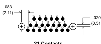
21 Contacts
