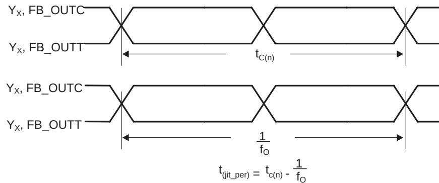
Figure 6. Period Jitter
