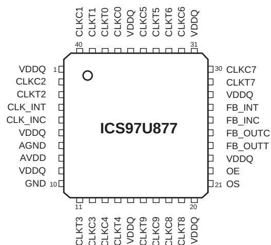
40-Pin MLF
