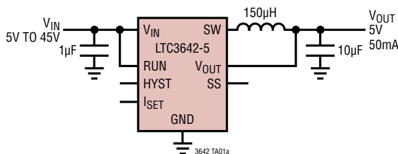
5V, 50mA Step-Down Converter
