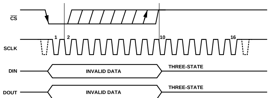
Figure 28. Entering Power-Down Mode
