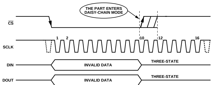
Figure 27. Entering Daisy-Chain Mode
