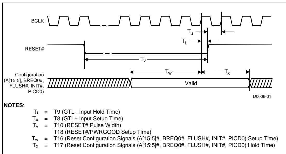
Figure 9. Cold/Warm Reset and Configuration Timings
