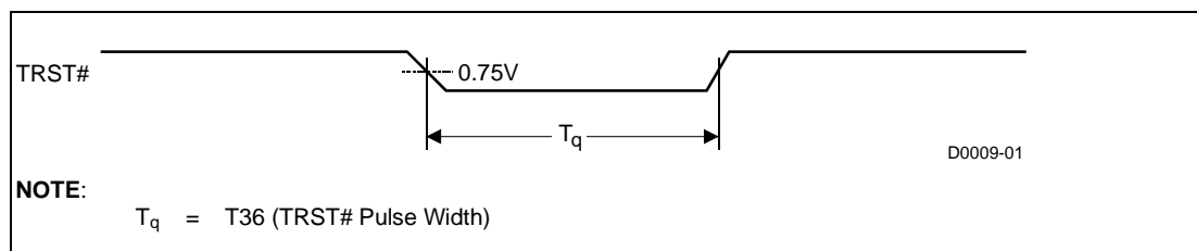
Figure 12. Test Reset Timings
