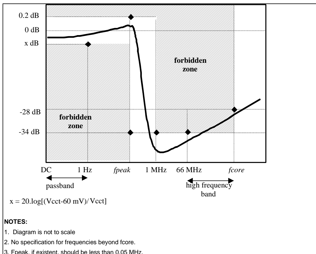
Figure 25. PLL Filter Specifications
