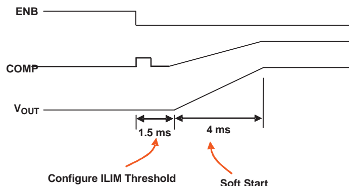
Figure 19. Startup
