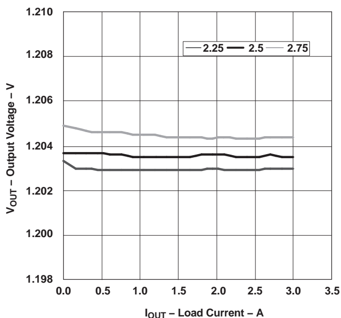
Figure 30. Typical Line/Load Regulation for 2.5-V to 1.2-V at 3-A Converter Using TPS40041
