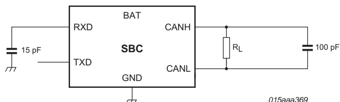
Fig 17. Timing test circuit for CAN transceiver
