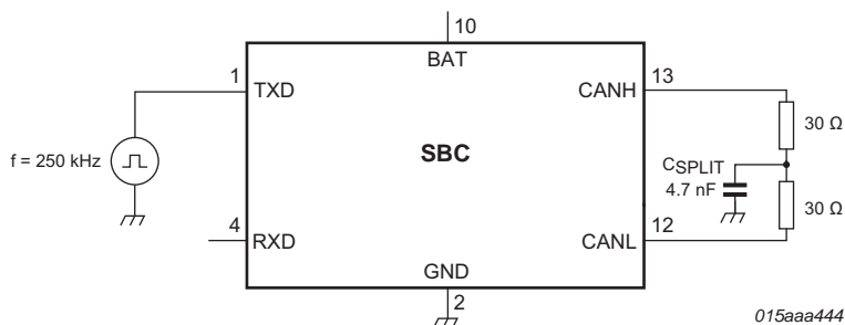
Fig 18. Test circuit for measuring transceiver driver symmetry
