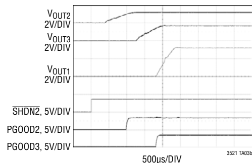
Sequenced Start-Up Waveforms
