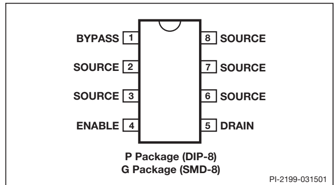
Figure 3. Pin Configuration.
