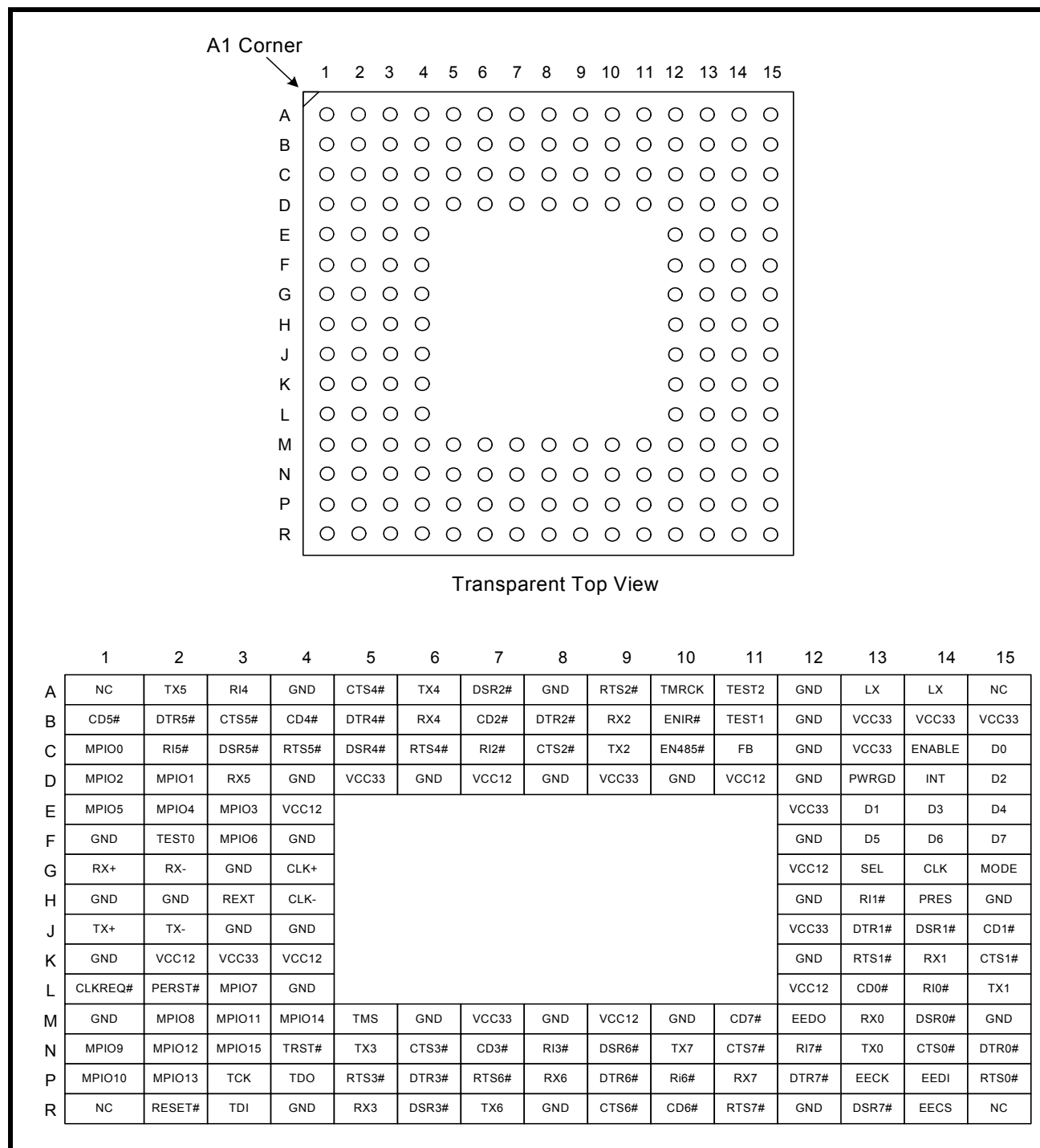
FIGURE 2. 176-FPBGA PINOUT
