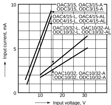
3. Input voltage and current (OAC, ODC)
