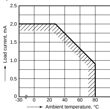
1-1. Load current vs. ambient temperature (OAC)
