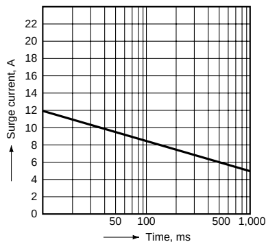
2-2. Surge current and time (IDC)
