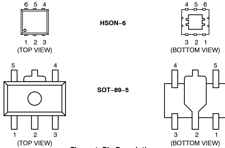
Figure 1. Pin Description
