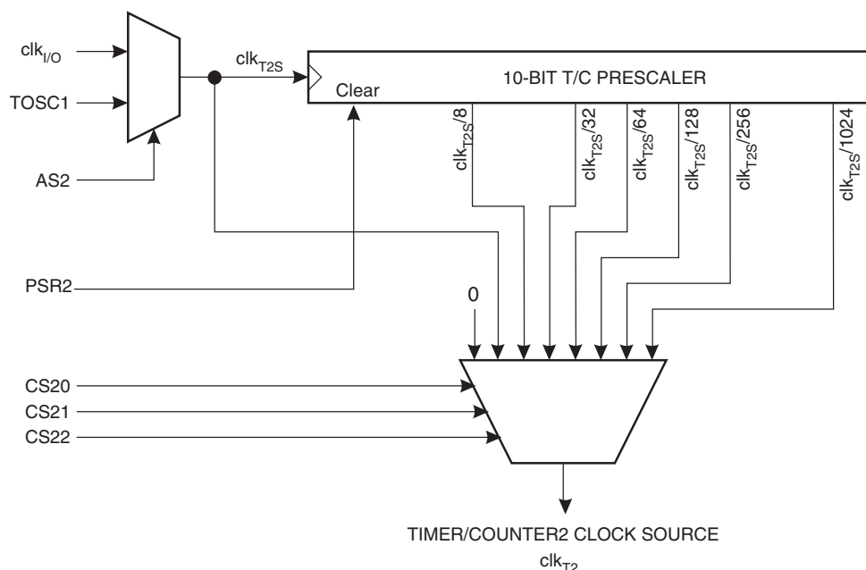
Timer/Counter Prescaler Figure 64. Prescaler for Timer/Counter2
