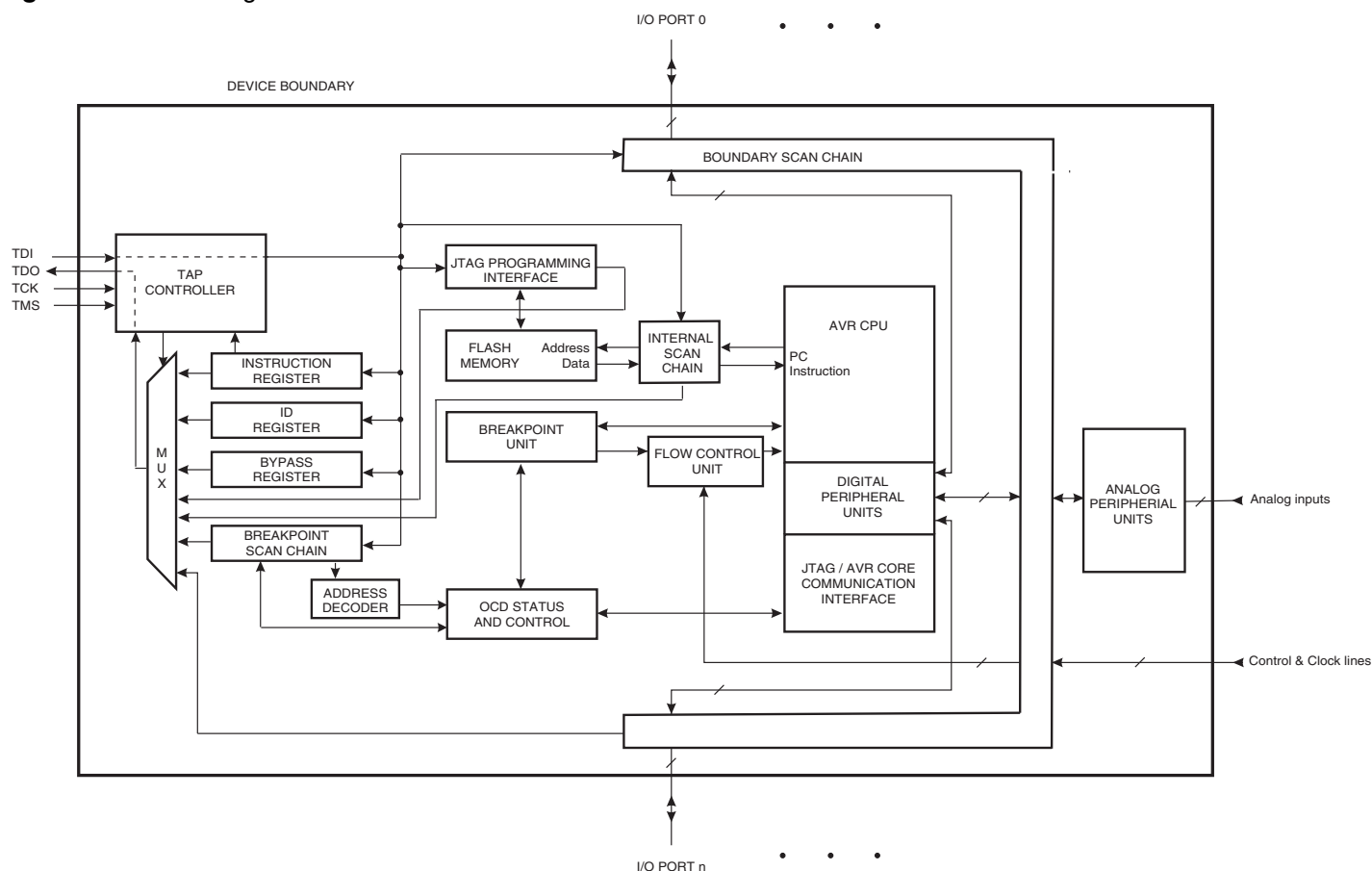
Figure 97. Block Diagram
