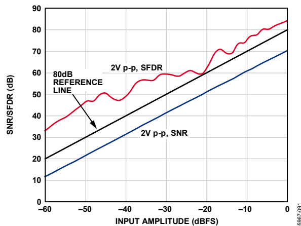
Figure 30. SNR/SFDR vs. Analog Input Level, f_{\text{IN}} = 10.3 MHz, AD9222-65
