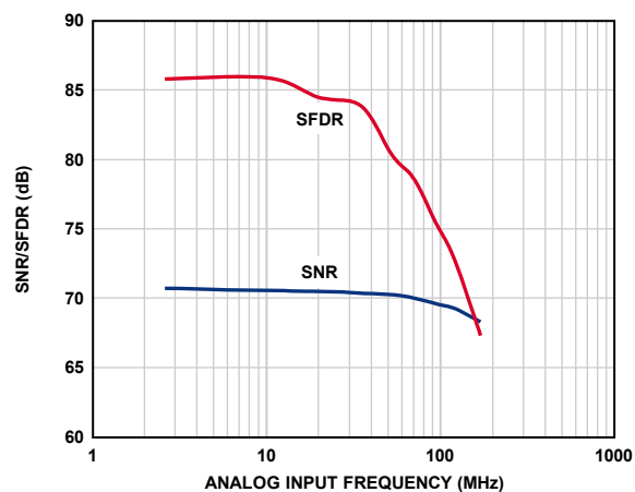
Figure 39. SNR/SFDR vs. f_{IN} , AD9222-50
