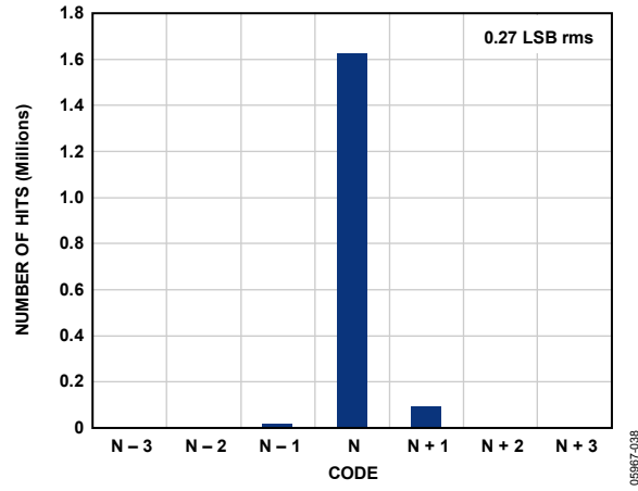
Figure 50. Input-Referred Noise Histogram, AD9222-50
