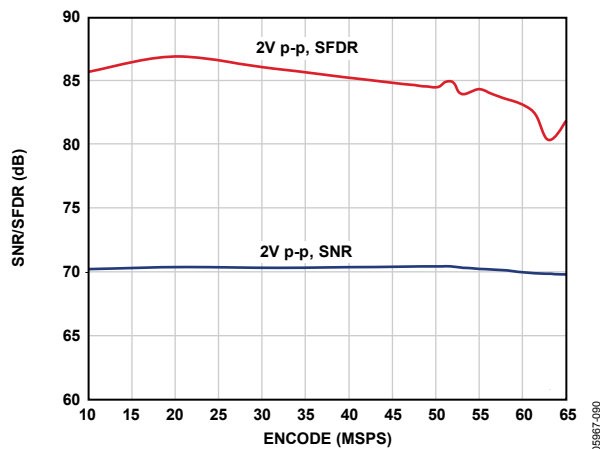
Figure 28. SNR/SFDR vs. f_{\text{SAMPLE}} , f_{\text{IN}} = 19.7 MHz, AD9222-65
