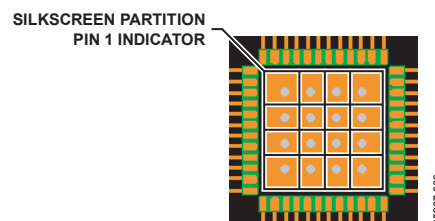
Figure 85. Typical PCB Layout
