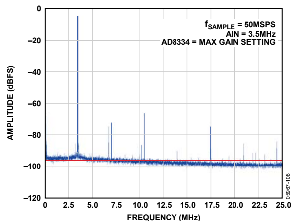
Figure 89. AD9222 FFT Example Results Using 16 MHz, Two-Pole Low-Pass Filter Applied to the AD8334 Outputs ( f_{\text{SAMPLE}} = 50\ \text{MSPS} , A_{\text{IN}} = 3.5\ \text{MHz} , AD8334 = Maximum Gain Setting, Analog Input Signal = -1.03\ \text{dBFS} , SNR = 60.8\ \text{dBc} , SFDR = 67.02\ \text{dBc} )
