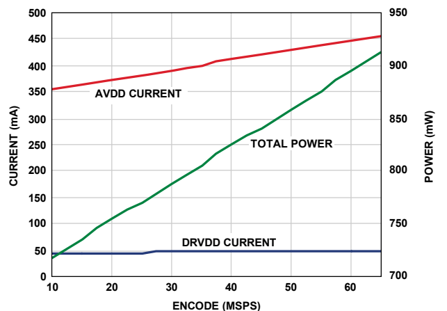
Figure 70. Supply Current vs. f_{\text{SAMPLE}} for f_{\text{IN}} = 10.3 \text{ MHz} , AD9222- 65
