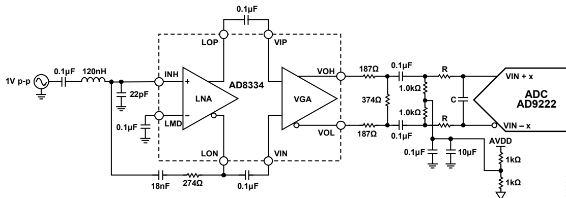
Figure 62. Differential Input Configuration Using the AD8334
