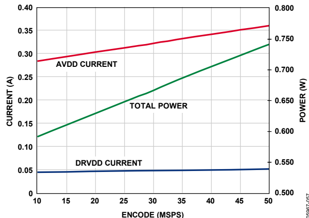
Figure 69. Supply Current vs. f_{\text{SAMPLE}} for f_{\text{IN}} = 10.3 \text{ MHz} , AD9222- 50
