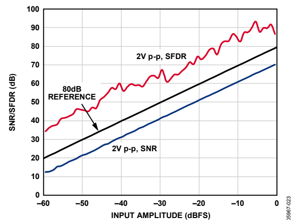
Figure 29. SNR/SFDR vs. Analog Input Level, f_{\text{IN}} = 10.3 MHz, AD9222-50
