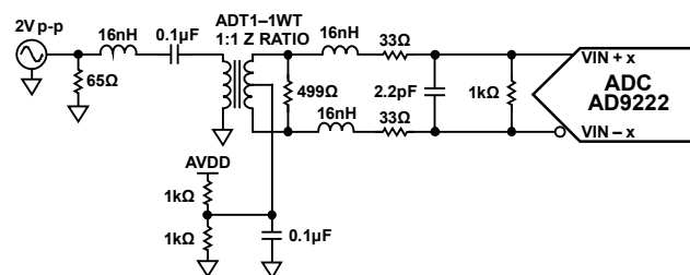
Figure 60. Differential Transformer-Coupled Configuration for IF Applications
