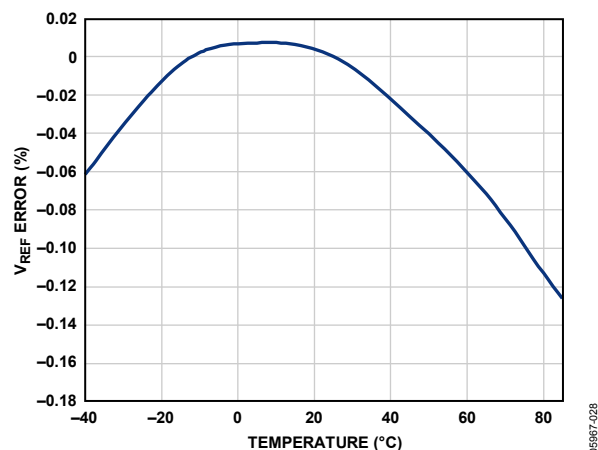
Figure 82. Typical V_{REF} Drift, AD9222-50
