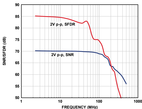
Figure 40. SNR/SFDR vs. f_{IN} , AD9222-65
