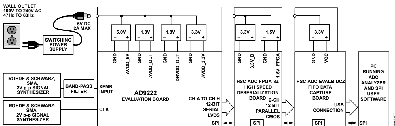
Figure 86. Evaluation Board Connection
