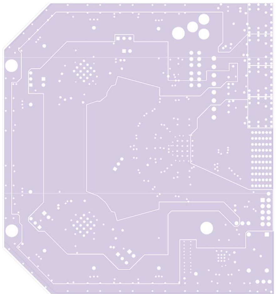
Figure 99. Evaluation Board Layout, Power Plane
