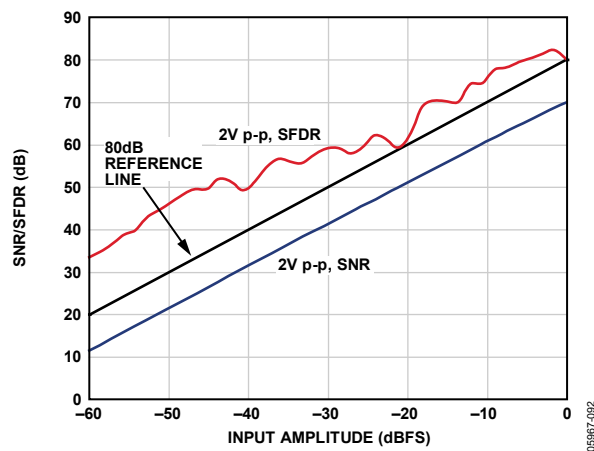
Figure 32. SNR/SFDR vs. Analog Input Level, f_{\text{IN}} = 35 MHz, AD9222-65
