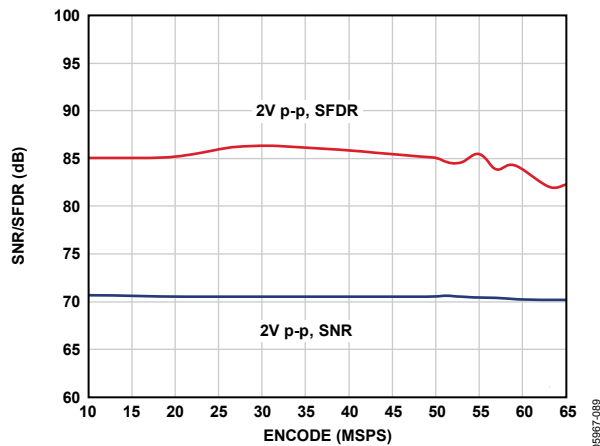
Figure 27. SNR/SFDR vs. f_{\text{SAMPLE}} , f_{\text{IN}} = 2.3 MHz, AD9222-65
