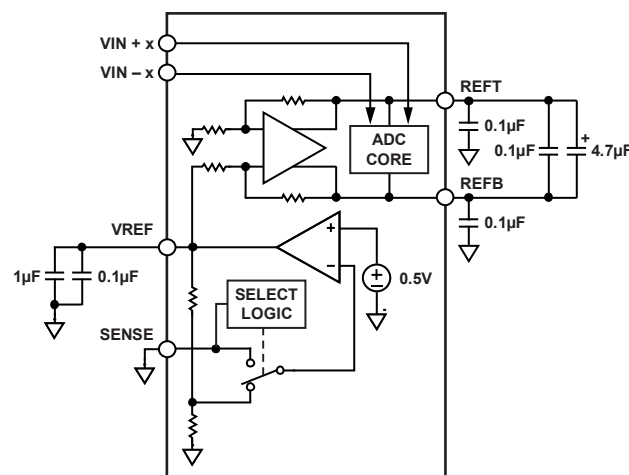
Figure 79. Internal Reference Configuration
