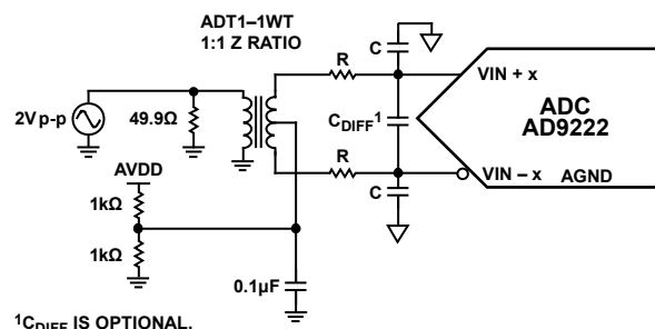
Figure 59. Differential Transformer-Coupled Configuration for Baseband Applications
