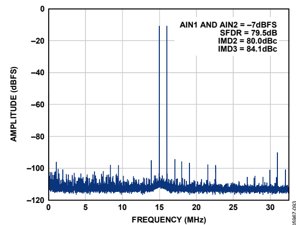
Figure 37. Two-Tone 32k FFT with f_{IN1} = 15 MHz and f_{IN2} = 16 MHz, AD9222-65
