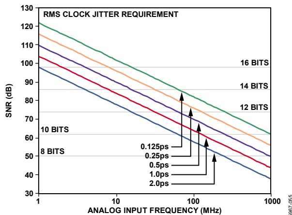
Figure 68. Ideal SNR vs. Input Frequency and Jitter
