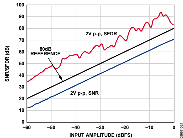
Figure 31. SNR/SFDR vs. Analog Input Level, f_{\text{IN}} = 35 MHz, AD9222-50
