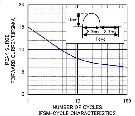
IFSM-CYCLE CHARACTERISTICS
