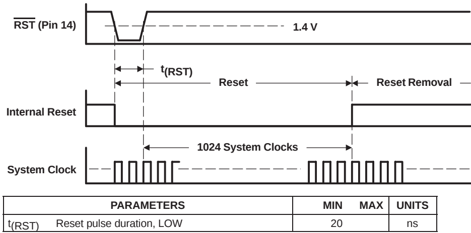
Figure 20. External Reset Timing
