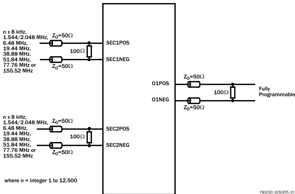
Figure 14 Recommended Line Termination for LVDS Input/Output Ports
