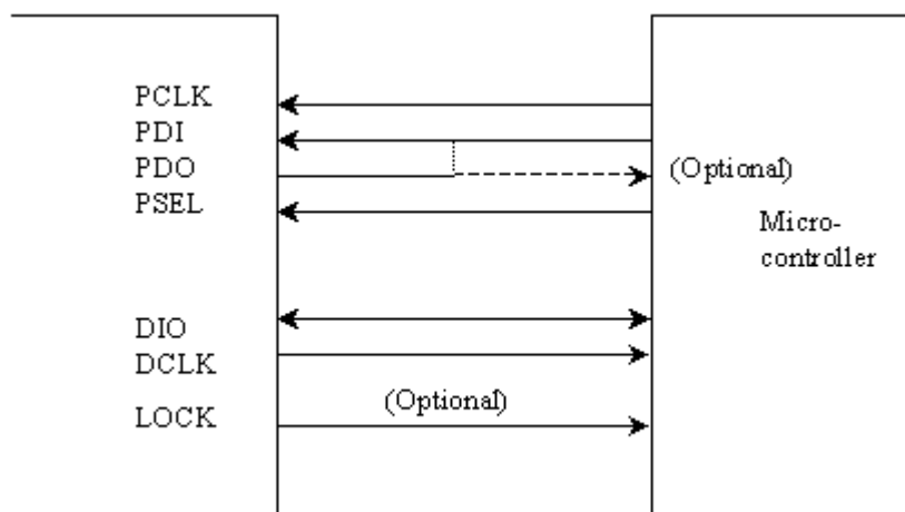
Figure 5-3. Microcontroller Interface
