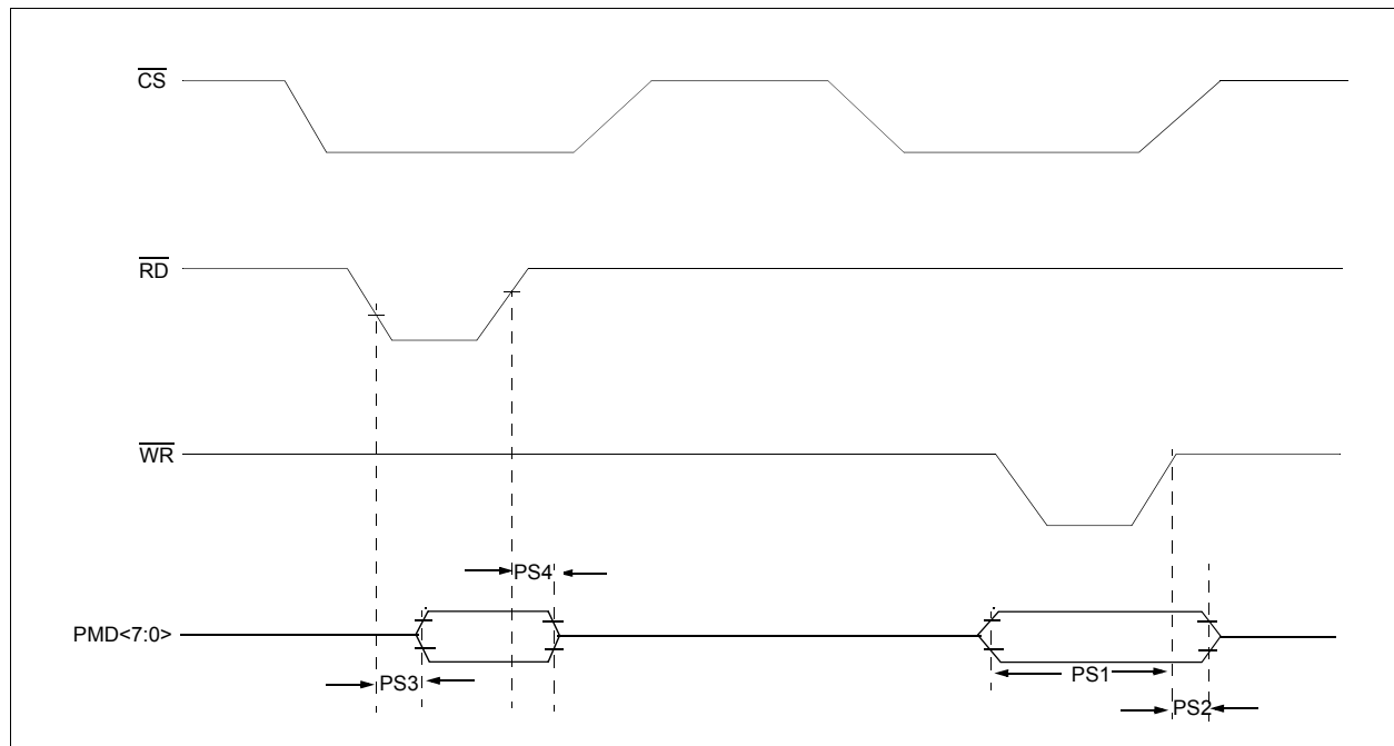
FIGURE 30-26: PARALLEL SLAVE PORT TIMING DIAGRAM
