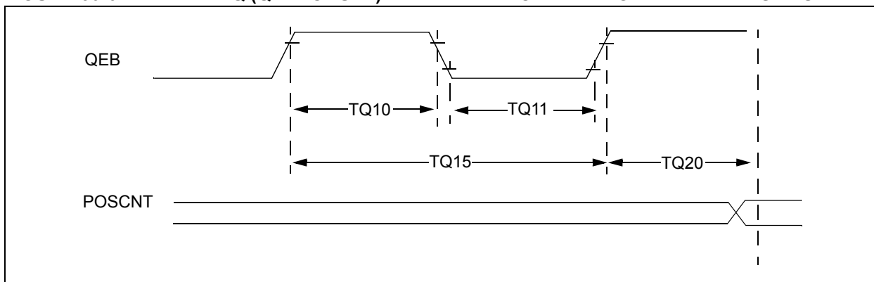
FIGURE 30-6: TIMERQ (QE1 MODULE) EXTERNAL CLOCK TIMING CHARACTERISTICS
