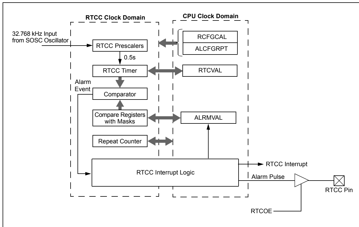
FIGURE 24-1: RTCC BLOCK DIAGRAM
