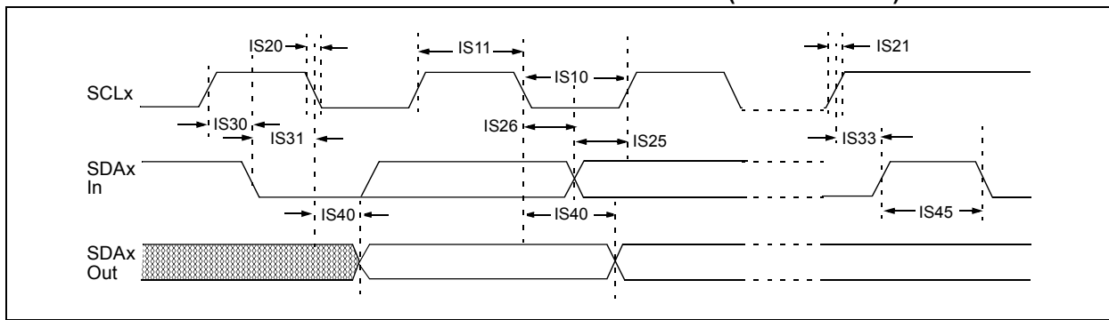
FIGURE 30-21: I2Cx BUS DATA TIMING CHARACTERISTICS (SLAVE MODE)
