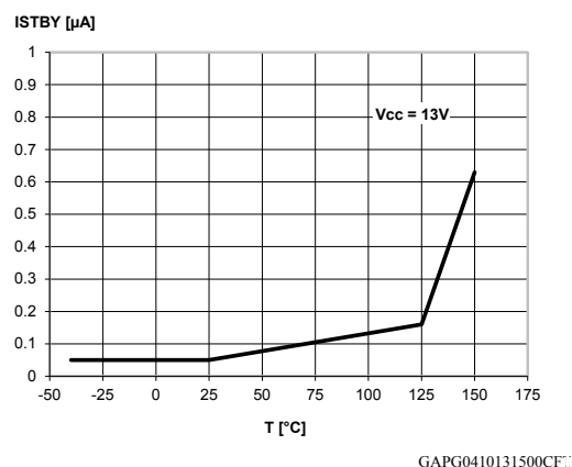
Figure 16. Standby current
