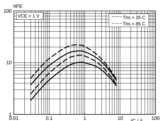
Fig.5. DC current gain. h_{FE} = f(I_C) Parameter T_{HS} (Low and high gain)
