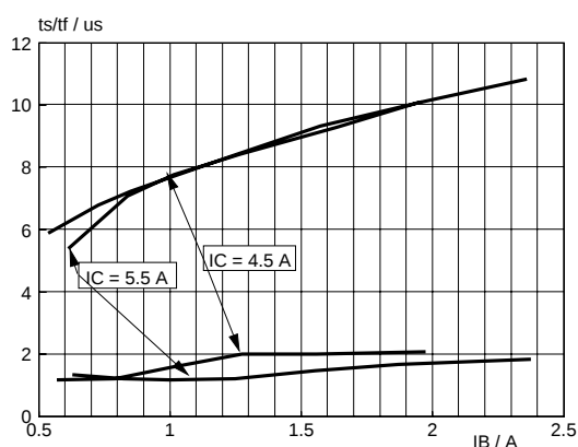
Fig.10. Limit storage and fall time. t_s = f(I_B) ; t_f = f(I_B) ; parameter I_C ; T_{HS} = 85^\circ\text{C} ; f = 16\text{ kHz}
