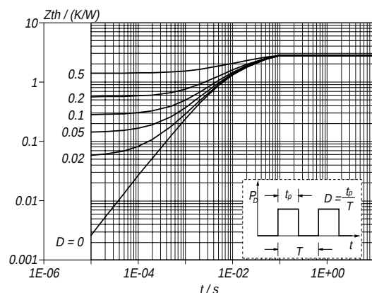
Fig.12. Transient thermal impedance. Z_{th \text{ j-hs}} = f(t) ; parameter D = t_p / T
