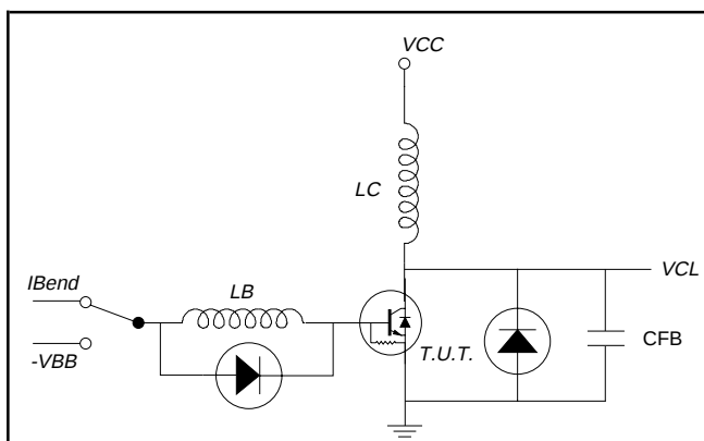
Fig.13. Test Circuit RBSOA. V_{CC} = 150 \text{ V} ; -V_{BB} = 1 - 4 \text{ V} ; L_C = 1 \text{ mH} ; V_{CL} = 1500 \text{ V} ; L_B = 1 - 3 \mu\text{H} ; C_{FB} = 1 - 4 \text{ nF} ; I_{B(end)} = 1.2 - 4 \text{ A}
