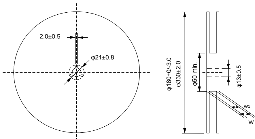
Fig.3 Taping Diagram
