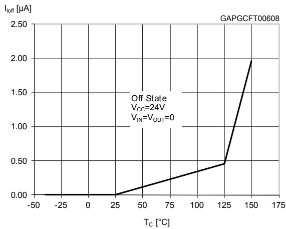
Figure 13. Off-state output current
