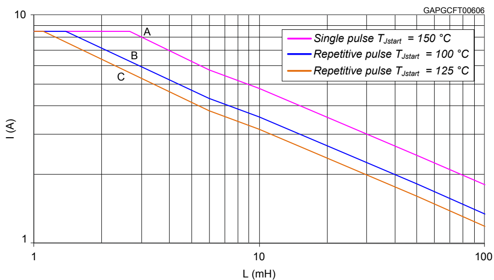
Figure 25. Maximum turn off current versus inductance
