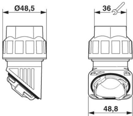
Dimensioned drawing
