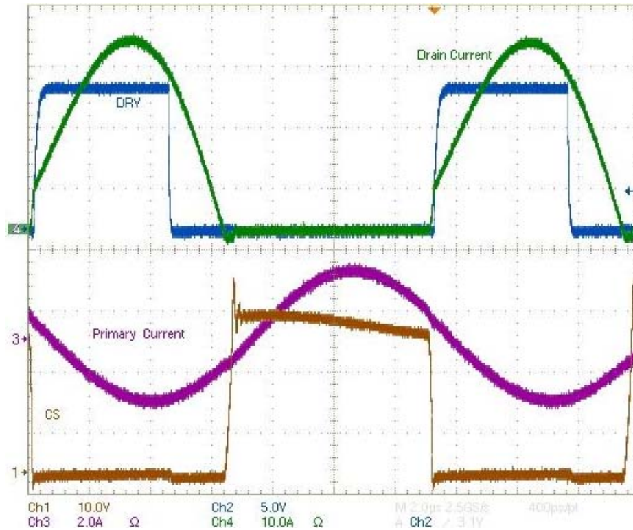
Figure 35. Waveforms from SR System Using MOSFET in TO220 Package without Parasitic Inductance Compensation – SR MOSFET Channel Conduction Time is Reduced
