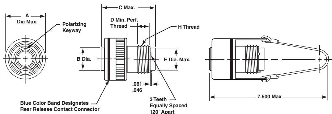
9818 Connector
