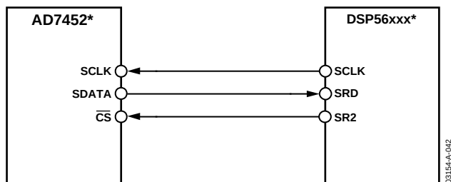
Figure 42. Interfacing to the DSP56xxx
