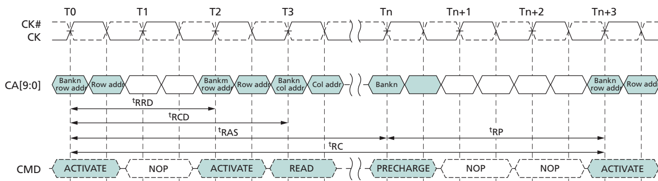
Figure 16: ACTIVATE Command
