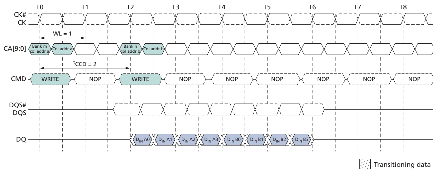
Figure 31: Seamless Burst WRITE – WL = 1, BL = 4, t_{CCD} = 2
