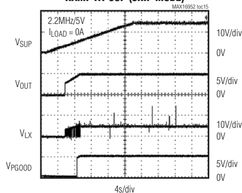
OUTPUT RESPONSE TO SLOW RAMP AT SUP (SKIP MODE)
