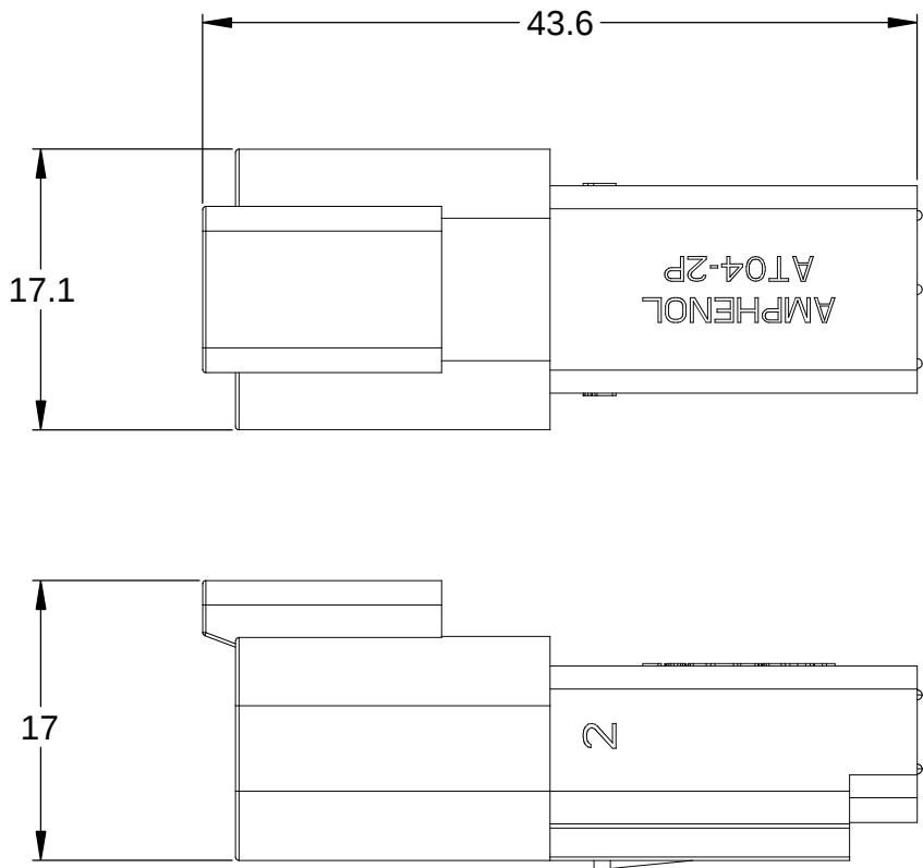
REFERENCE DIMENSIONS - ASSEMBLED
