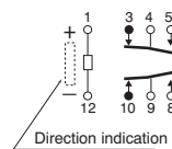
Schematic (Bottom view) Single side stable
